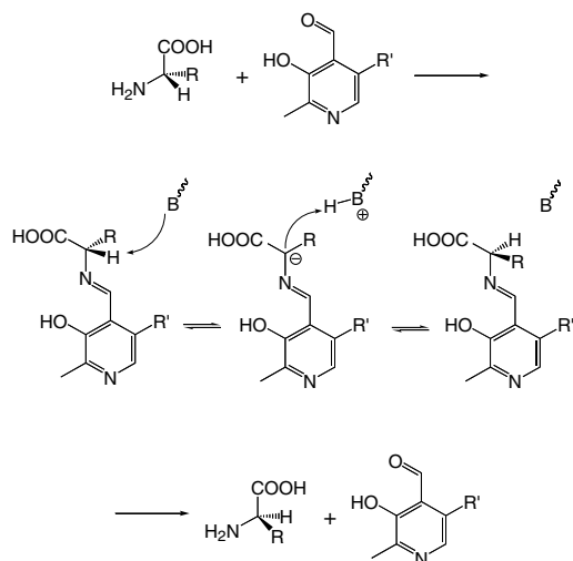
Figure 6. Racemization of \alpha -amino acid catalyzed by pyridoxals.
