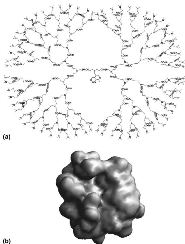
Figure 5. Chemical structure (a) and three-dimensional view (b) of the G6-Me PAMAM–pyridoxal molecule.
