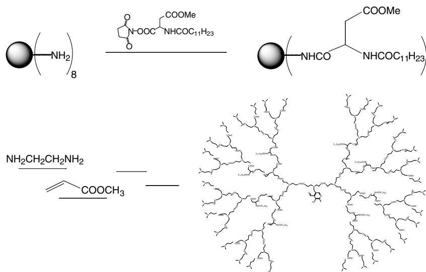
Figure 8. Synthesis of dendrimeric PAMAM-pyridoxals carrying eight internal lauryl groups.
