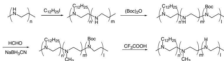
Figure 2. The synthesis of PEI polymers with only about 2% primary or secondary amino groups.
