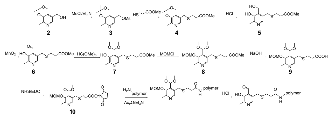
Figure 1. The synthesis of polymeric PEI-pyridoxals.
