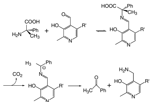
Figure 7. Decarboxylation of 2-amino-2-phenyl-propionic acid mediated by pyridoxals.
