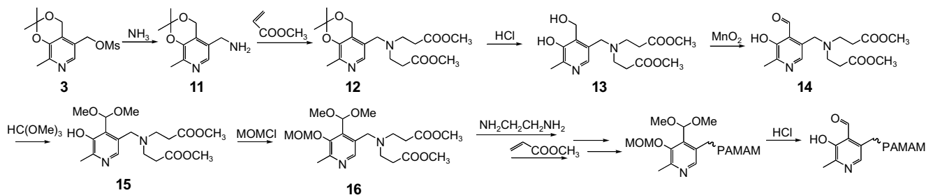
Figure 4. Synthesis of dendrimeric PAMAM–pyridoxals.
