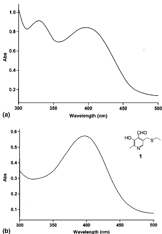
Figure 3. The UV spectrum of (a) the laurylated polymeric PEI–pyridoxal, and (b) of a simple pyridoxal compound, that is 5-[[ethythio)methyl-3-hydroxy-2-methyl-4-pyridinecarbaldehyde] ( 1 ).
